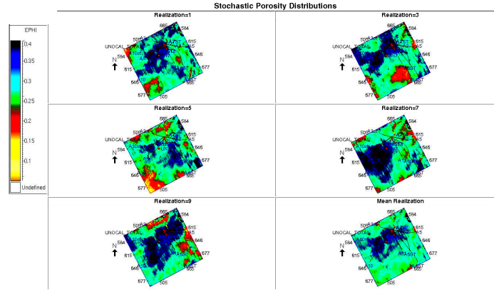
Fig. 3. Plan view of the spatial distribution of porosity obtained with geostatistical inversion of well logs and 3D post-stack seismic data. From left to right, and from top to bottom, realizations no. 1, 3, 5, 7, 9 and the mean of 10 realizations.
