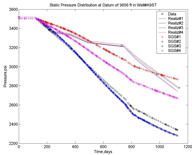
Fig. 4. Time evolution of static pressure in well A9ST after the onset of production. Solid lines describe pressures simulated from reservoir models constructed with geostatistical inversion. Dashed lines describe pressures simulated from reservoir models constructed with SGS.
